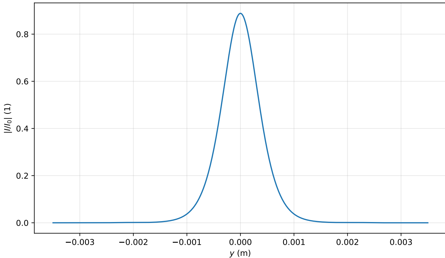
Intensity profile I(x=0, y, z=3.901)/I_0 , P_{in}=0.8P_{cr} , artificial time
